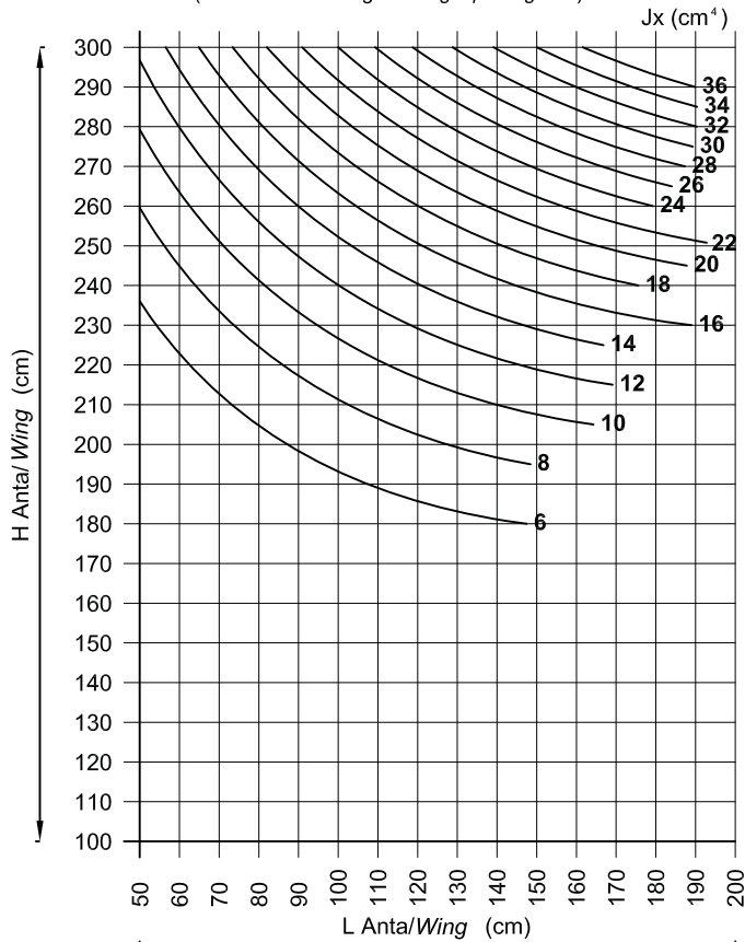
CARICO DEL VENTO/ WIND LOAD : q= 50 Kg/m 2 f max H/200 (Vetro in lastra singola/ Single pane glass)
